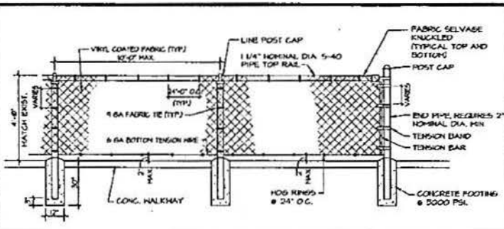
7 | CHAIN LINK FENCE DETAIL SCALE: 1/2" = 1'-0"
